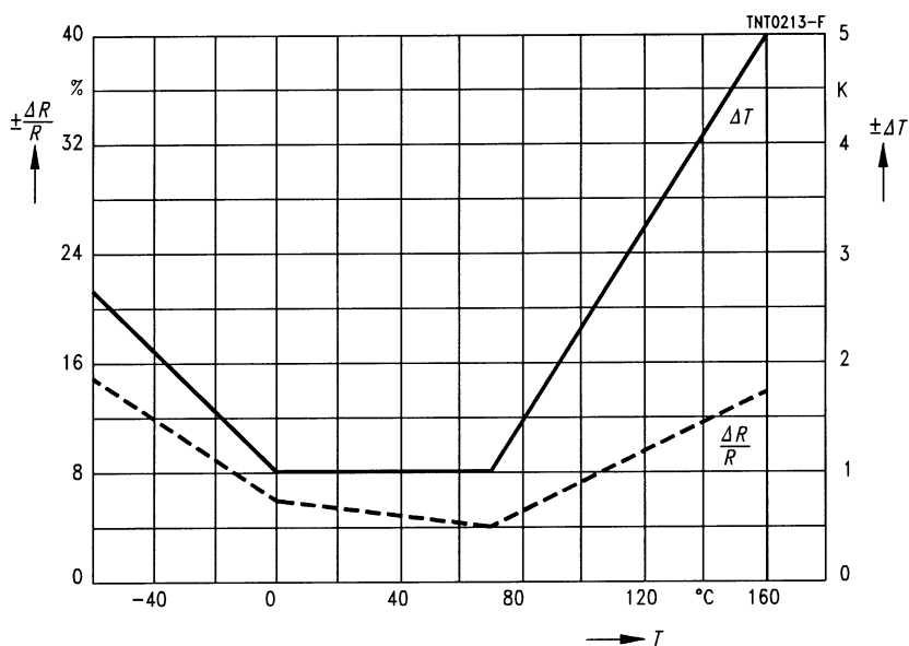
Resistance and temperature tolerances versus temperature ( \Delta T = 1 K)
