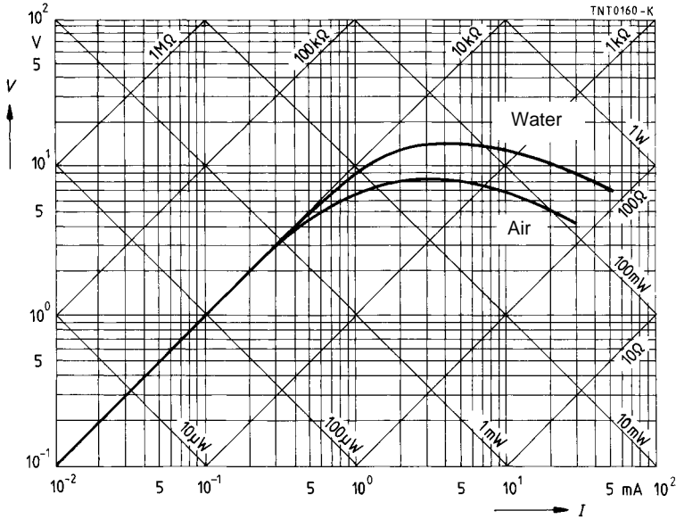
Figure 3 Current/voltage characteristic
